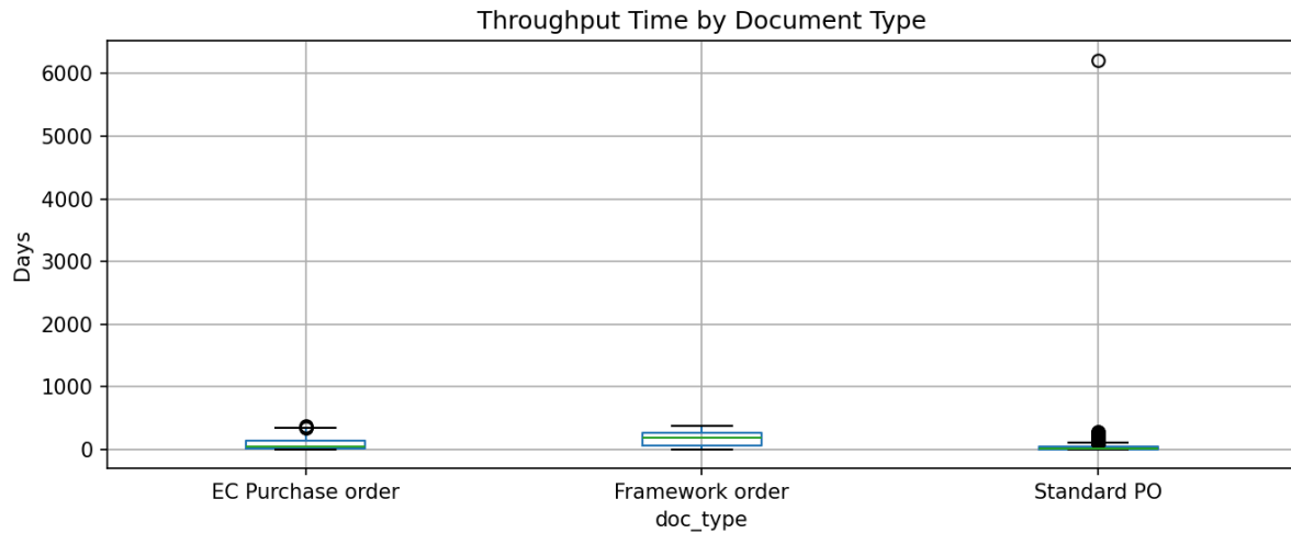
Figure 7: Throughput time distribution by document type (cDocType) for the BPI Challenge 2019 sample. Each box shows the interquartile range; whiskers extend to 1.5 times the IQR. Standard PO cases show a wider spread and longer tail compared with Framework order cases, reflecting the greater process complexity of standard purchase orders that require three-way matching.
