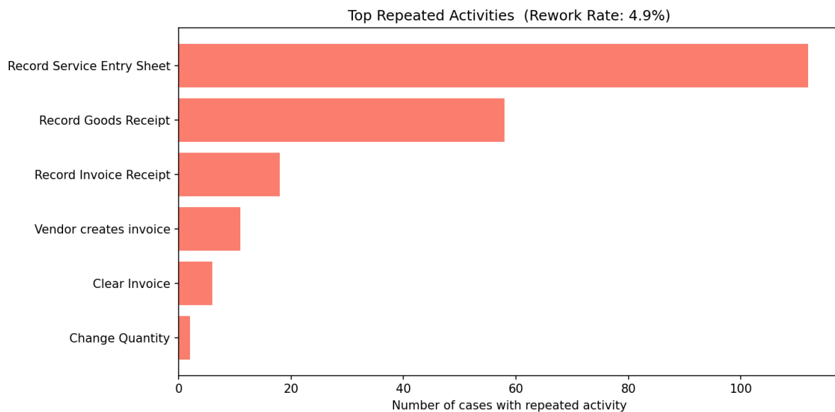
Figure 4: Top activities by rework occurrence in the BPI Challenge 2019 dataset. Each bar shows the number of cases in which the activity was observed more than once within a single case. Record Service Entry Sheet is the most frequently repeated activity, appearing with count greater than one in 112 cases, confirming that service entry correction cycles are the dominant source of rework in the procurement process.
