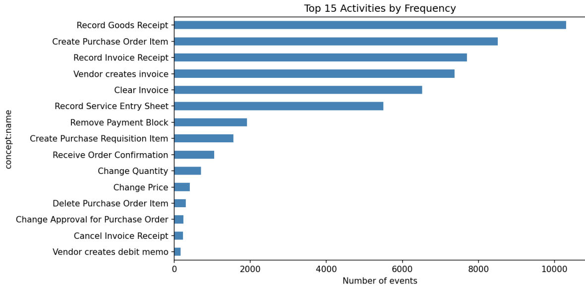
Figure 1: Activity frequency distribution for the BPI Challenge 2019 dataset (training set of 37,238 cases, 70% of the full log). Activities are ranked by total occurrence count. Mandatory steps such as goods receipt and invoice verification dominate, while exception-handling activities appear at much lower frequencies.
