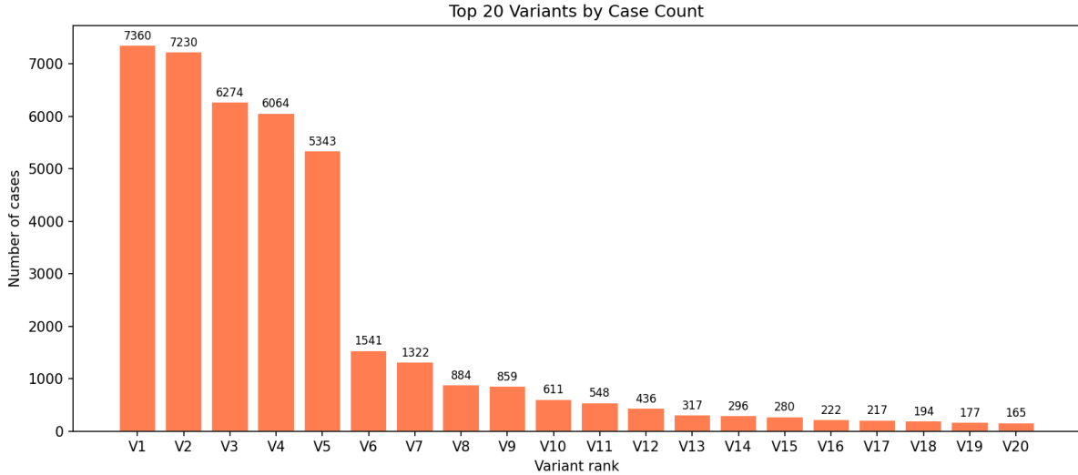
Figure 3: Variant frequency distribution for the BPI Challenge 2019 sample. The horizontal axis shows variant rank ordered by decreasing frequency and the vertical axis shows the number of cases per variant. A small number of variants account for the majority of cases, while the long tail contains many variants observed only once or a few times.
